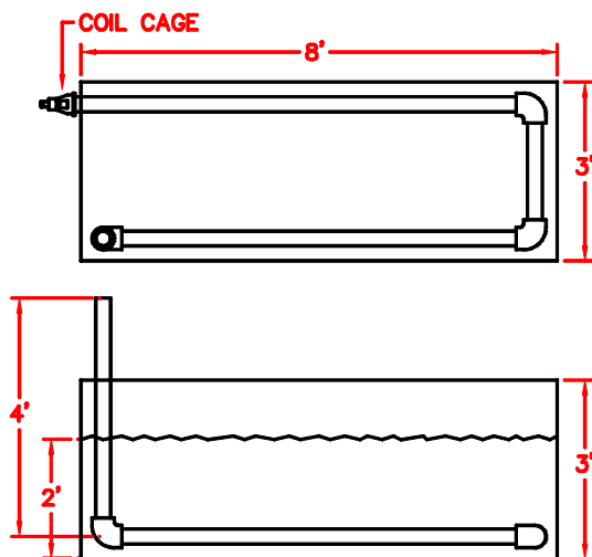
FIGURE 2 EXAMPLE : SELECTION OF IMMERSION COIL AND BURNER
