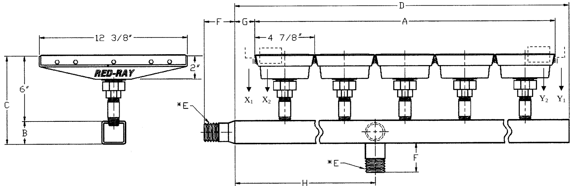
BURNER DIMENSIONS IN INCHES
