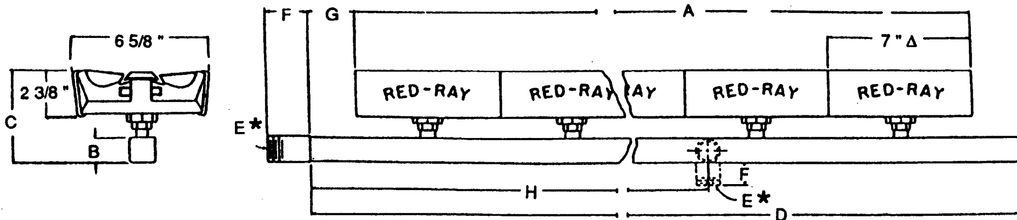
BURNER DIMENSIONS IN INCHES
